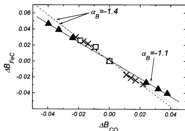
FIGURE 6 The correlation between the calculated changes in B_{FeC} and B_{CO} caused by the appearance of the different proximal Q_4 (×) and equatorial Q_3 (▲) point charges and changes of the tautomeric form and orientation of the distal histidine (□).
