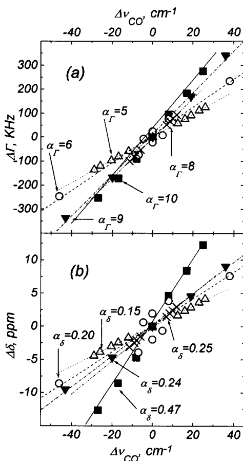
FIGURE 8 The correlation between the calculated values of \Delta\Gamma and \Delta\nu_{\text{CO}} (a), and \Delta\delta and \Delta\nu_{\text{CO}} (b) caused by the distal Q_1 (■) and Q_2 (○), equatorial Q_3 (×), and proximal Q_4 (△) point charges and homogeneous electric field (▲).
